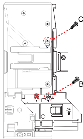
Unextended Connector Plate (6865i)
