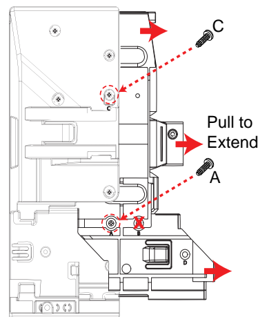
Extended Connector Plate (6867i/6869i)
